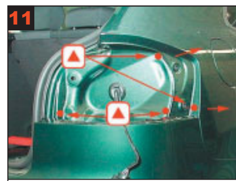
Rear wing/rear panel: 4 drill holes for correct treatment. Rear wing: Treat with lance.
