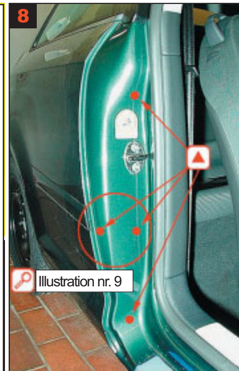
B-pillar and rear wing: Treat via 4 drilled holes for correct treatment. See fig 9 for drilling at correct level.
