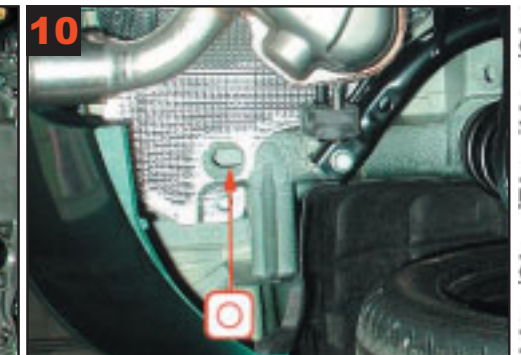
10 Longitudinal member rear: Treat via existing holes.
