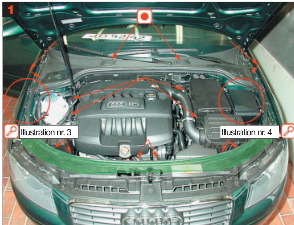
Engine compartment: Cowl: Treatment via existing plugged holes for washer. Flip plastic plate, treat with caution in underneath. Treat on top of longitudinal members, under airfilter box, engine suspension right side, reinforcements on spring strut right side. Treat locking plate. See fig 3 and 4 for correct treatment.
